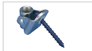
Branch Line Restraint Structure Attachment to Wood/Concrete (No seismic approval in concrete) CSBBS2EG
