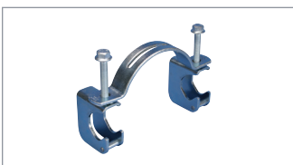
Quick Grip Lateral Sway Brace ("QG") CSBQG###EG
